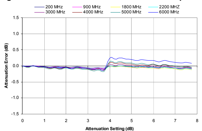
Figure 6. 0.25 dB Attenuation Error vs. Frequency
